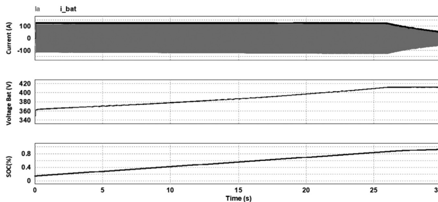
Fig. 3. Fast charging station behavior.
