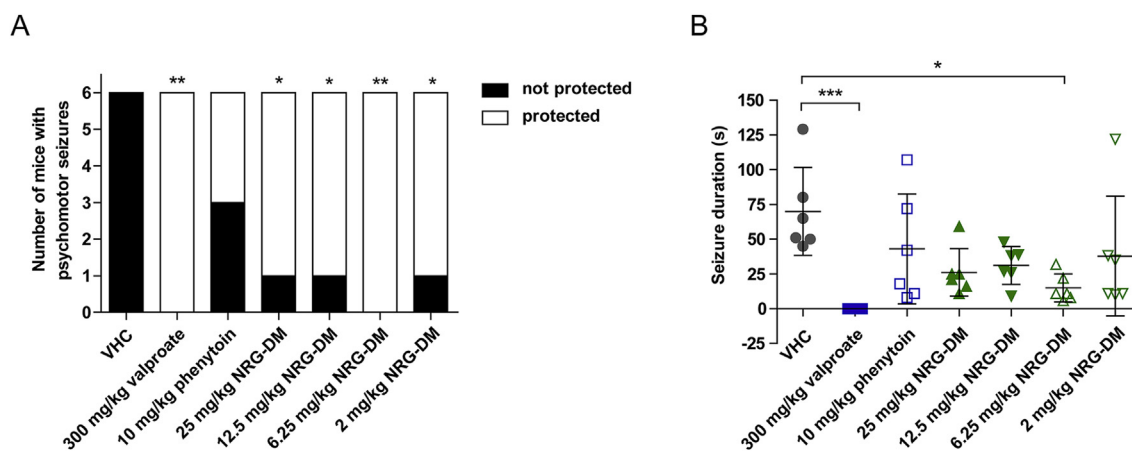
Fig. 4. Evaluation of the anti-seizure activity of naringenin 4',7-dimethyl ether (NRG-DM) in the mouse 6-Hz psychomotor seizure model. Drug-resistant focal seizures were induced by electrical stimulation (6 Hz, 0.2 ms rectangular pulse width, 3 s duration, 44 mA) through the cornea, 30 min after i.p. injection of vehicle (VHC, n = 6 ), positive control valproate ( n = 6 ), or NRG-DM ( n = 6 per dose), and 120 min after i.p. injection of negative control phenytoin ( n = 6 ). Number of mice protected against seizures are depicted (A) and defined by a seizure duration shorter than 40 s (s) (B). Data is shown as the mean \pm SD. Statistical analysis: (A) Fisher's exact test, (B) Kruskal-Wallis test with Dunn's multiple comparison test (GraphPad Prism 5). Significance levels: * p \leq 0.05 ; ** p \leq 0.01 ; *** p \leq 0.001 .
