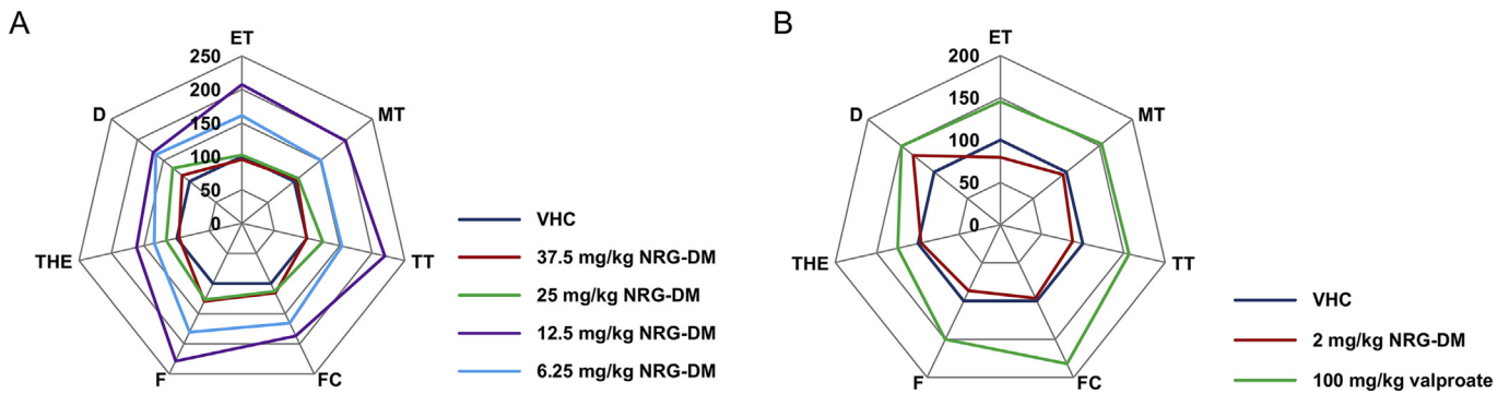
Fig. 3. Evaluation of the anti-seizure activity of naringenin 4',7-dimethyl ether (NRG-DM) in the mouse timed i.v. pentylenetetrazole (PTZ) seizure model. Radar graphic depicts mean PTZ doses required to induce seven characteristic behavioral parameters (ear twitch (ET), myoclonic twitch (MT), tail twitch (TT), forelimb clonus (FC), falling (F), tonic hind limb extension (THE), and death (D)), normalized to 100% for vehicle (VHC)-treated controls. VHC ( n = 8 (A) and 7 (B)), NRG-DM ( n = 5 per dose), and positive control valproate ( n = 5 ) were i.p. injected 30 min prior to continuous i.v. PTZ infusion.
