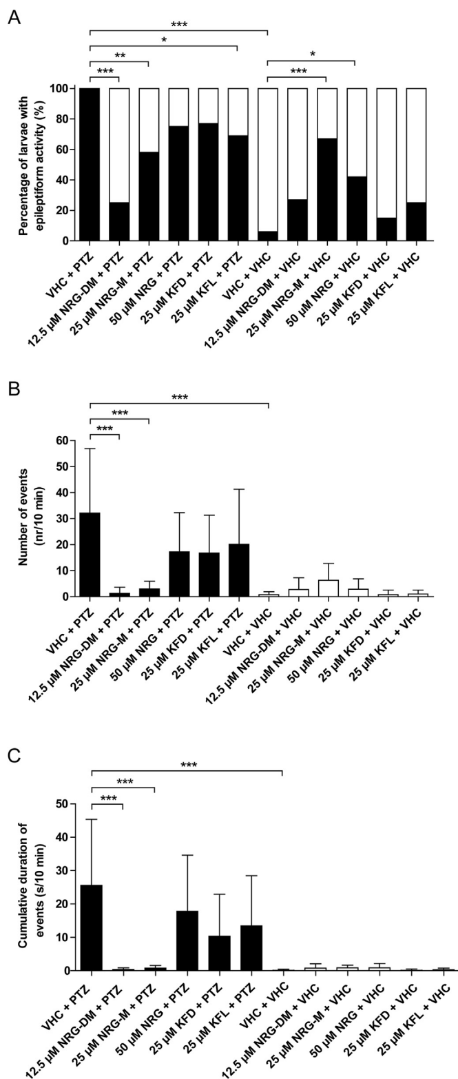
Fig. 2. Electrophysiology-based anti-seizure analysis of naringenin 4',7-dimethyl ether (NRG-DM), naringenin 7-O-methyl ether (NRG-M), naringenin (NRG), kaempferide (KFD), and kaempferol (KFL) in the zebrafish pentylenetetrazole (PTZ) seizure model. Non-invasive local field potential recordings from the optic tectum of larvae pre-exposed to vehicle (VHC) and PTZ (VHC + PTZ, n = 19 ), VHC only (VHC + VHC, n = 17 ), compound and PTZ ( n = 12 ), or compound and VHC ( n = 11-12 ). Larvae were pre-incubated with compound or VHC for 1 h, approximately. (A) Larvae are considered to show epileptiform brain activity when three or more epileptiform events occurred during a 10-min recording. Epileptiform discharges are quantified by the number (B) and cumulative duration (C) of events per 10-min recording. Data is
